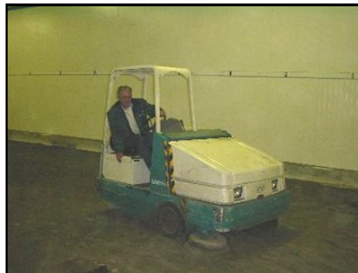
Surface preparation was carried out with rotating abrasive wheel equipment
